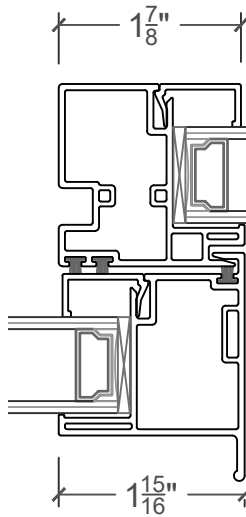
4 Meeting Rail Detail
